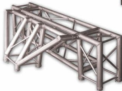
PK-710 / PK-1010 Top head truss piece for PIRAM-750 / 1000
